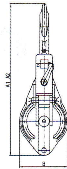
Single Sheave (SE/SH)
